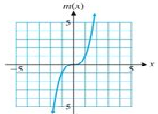
(C) Cube function m(x) = x^3 Domain: \mathcal{R} Range: \mathcal{R}
