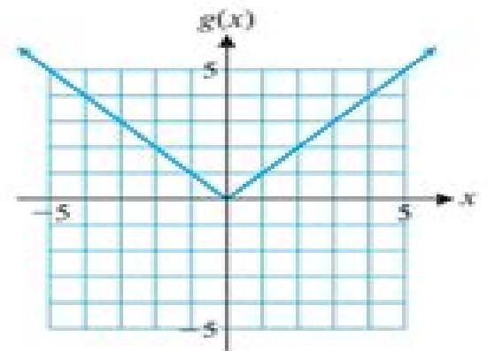
(F) Absolute value function g(x) = |x| Domain: \mathcal{R} Range: [0, \infty)
