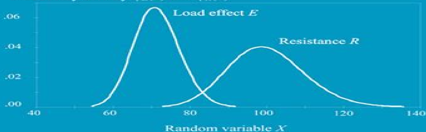
Probability density \varphi_E(x) and \varphi_R(x)
