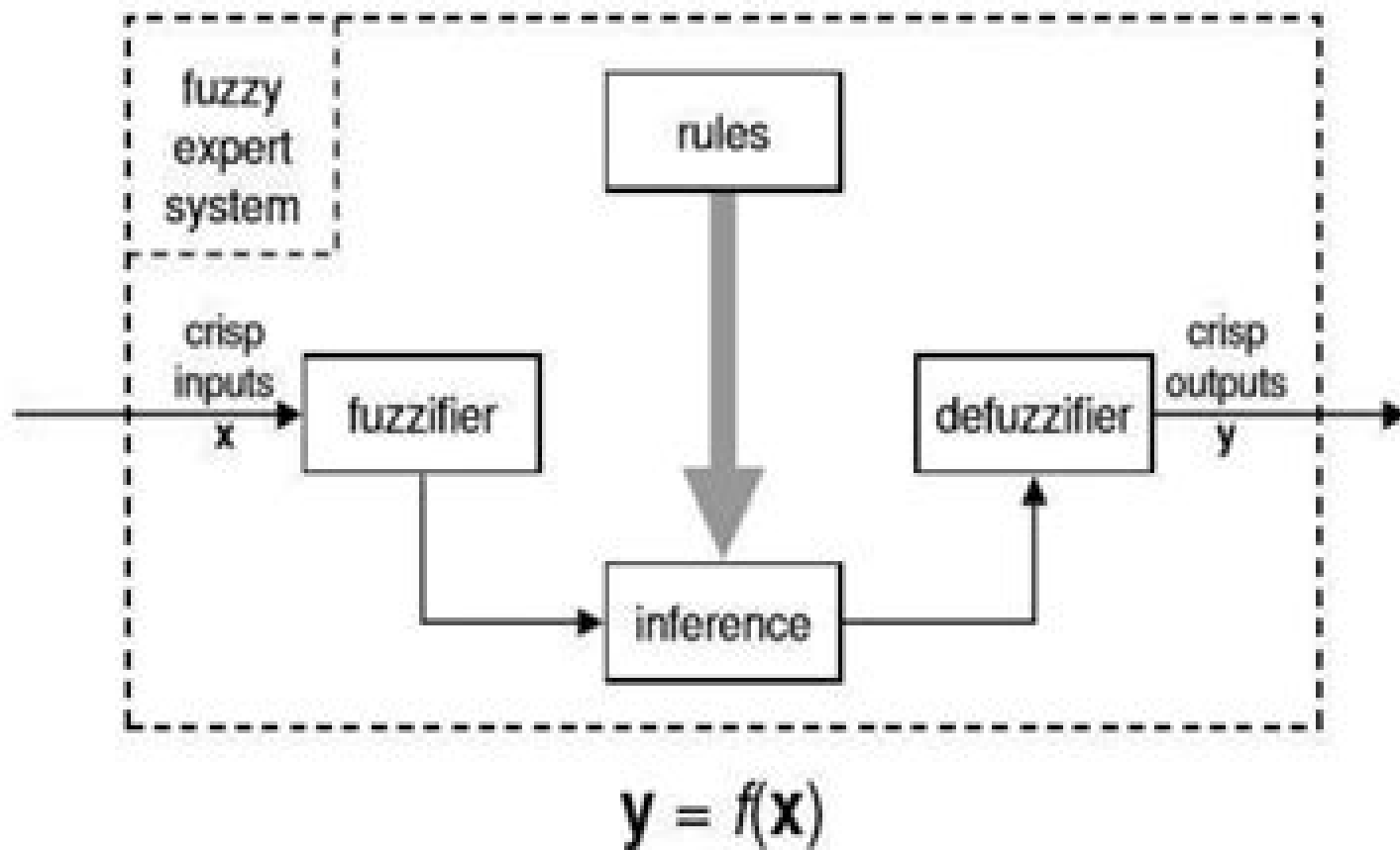
Fig. Generalized architecture of Fuzzy Expert system
