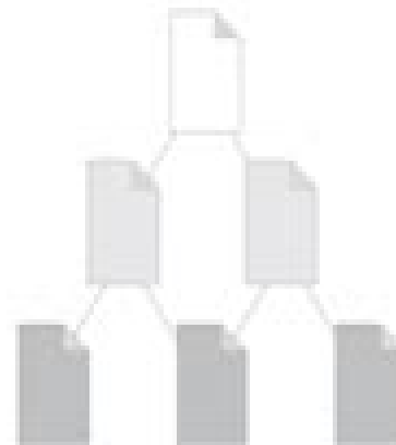
Document
