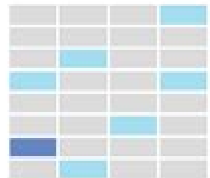
Wide Column
