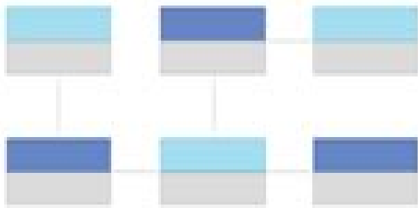
Relational
