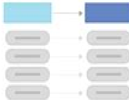
Key - Value
