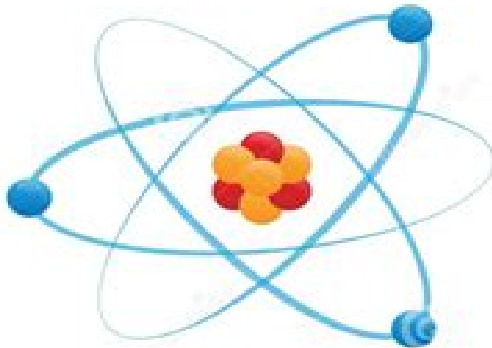
Bohr Model Electron Orbits
