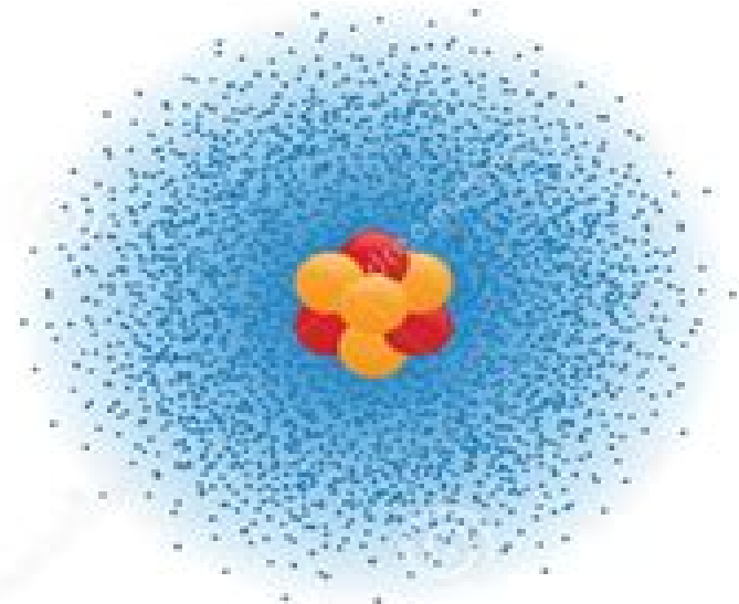
Quantum Mechanical Model Electron Clouds (Orbitals)
