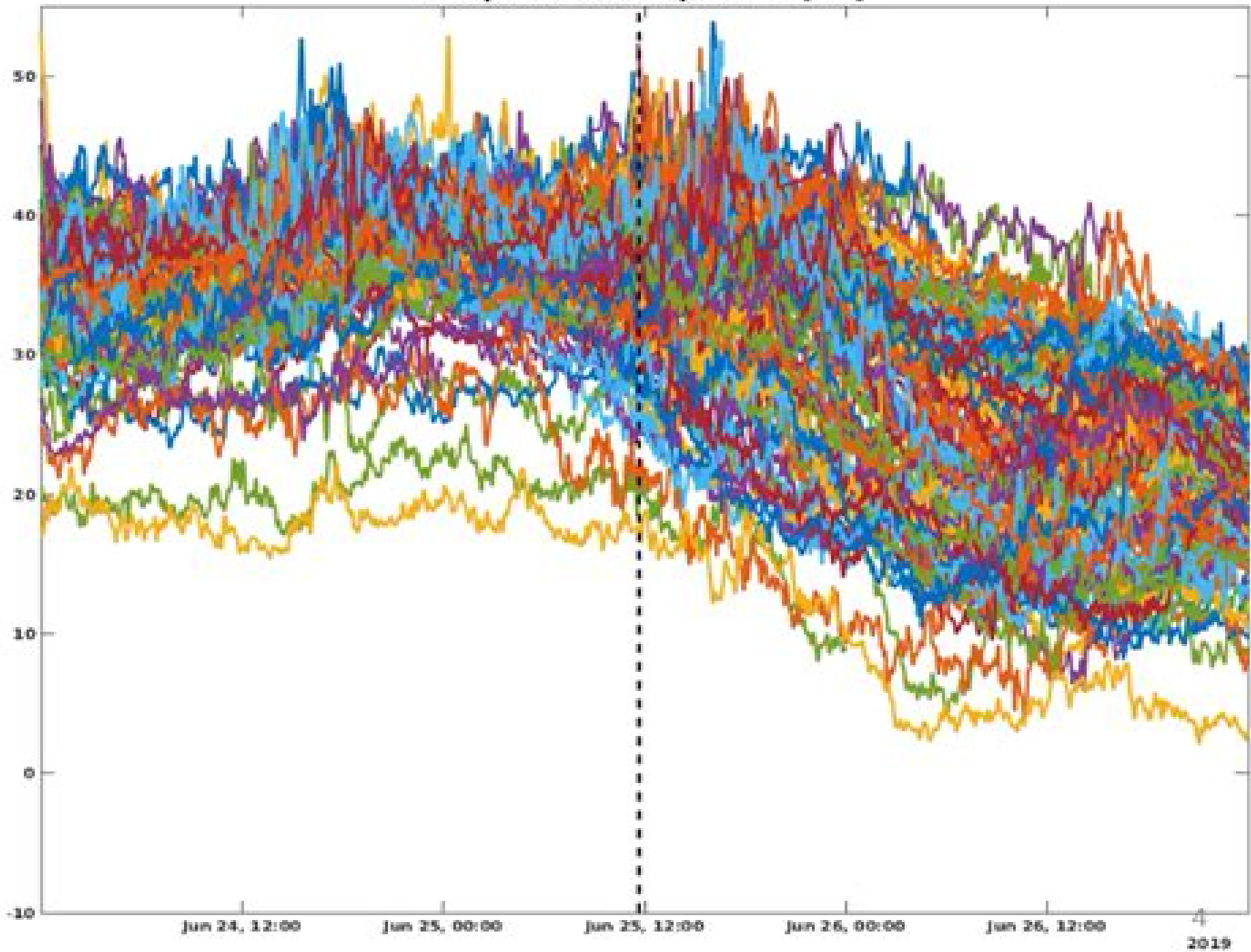
Precipitable Water Vapour PWV [mm]
