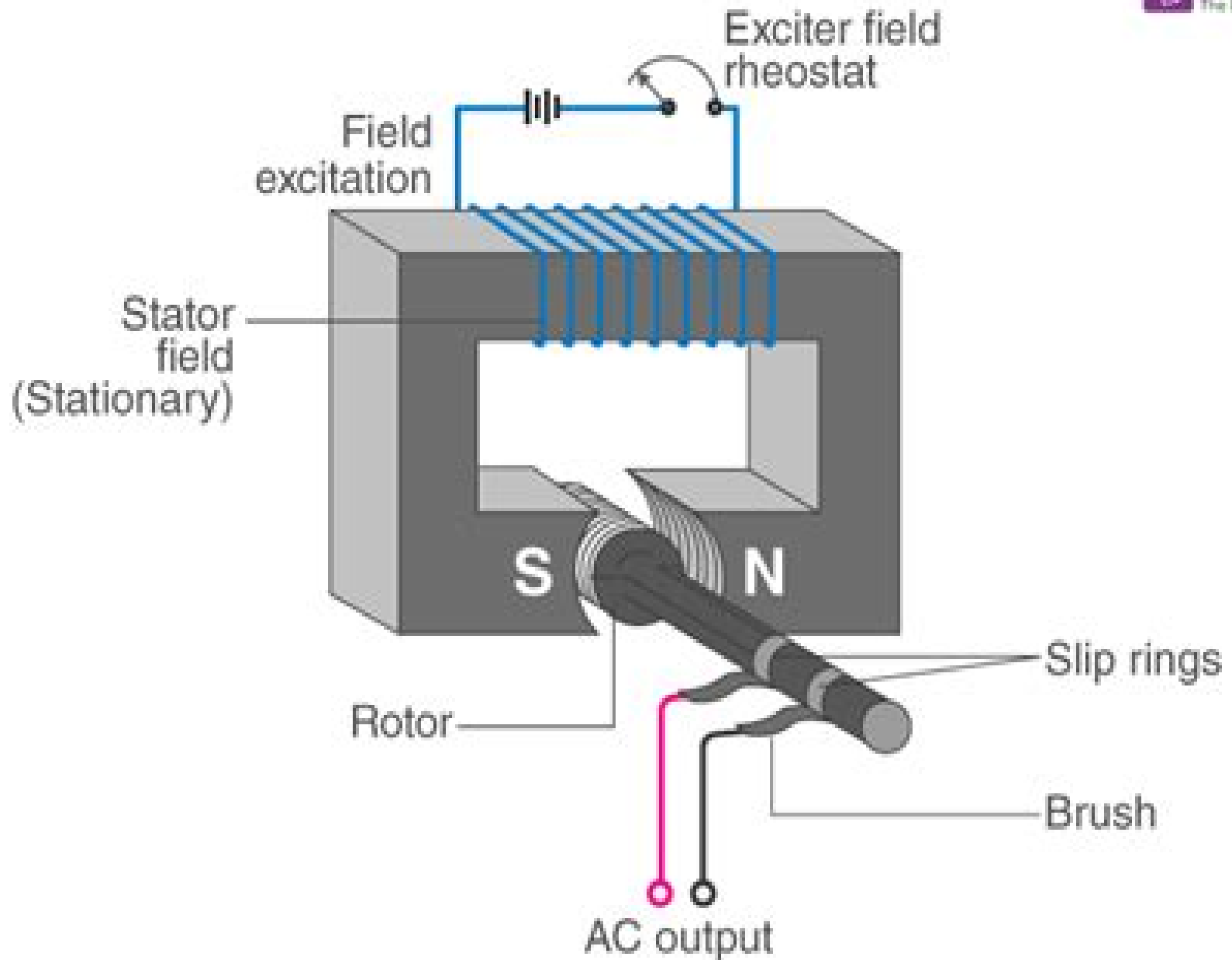
Basic AC Generator
