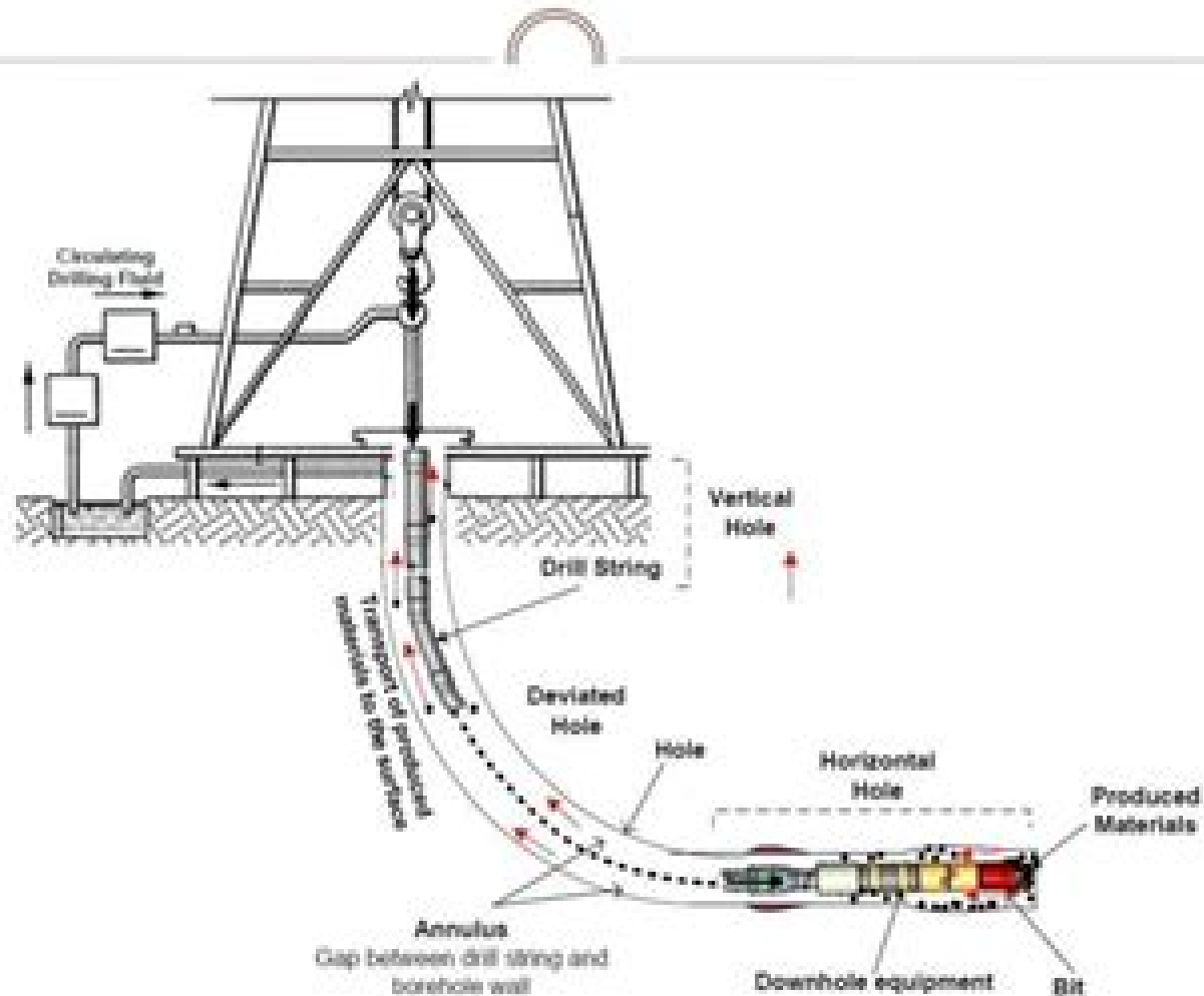
Fig. 1. Schematic drawing of an oil well being drilled.
