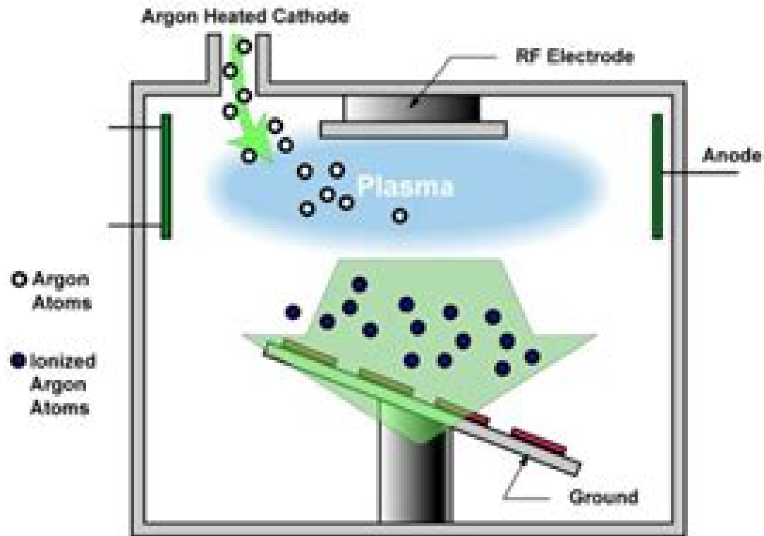
Ion Beam Milling
