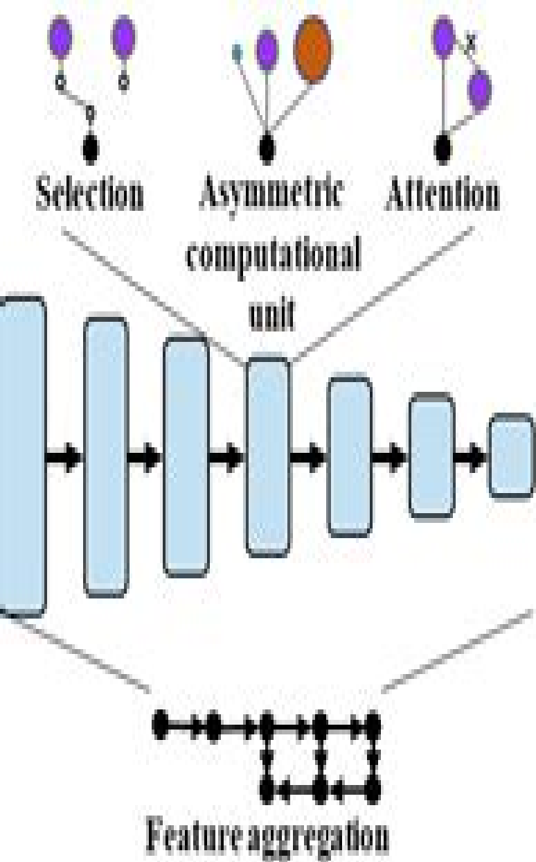
(a) Data path design strategies
