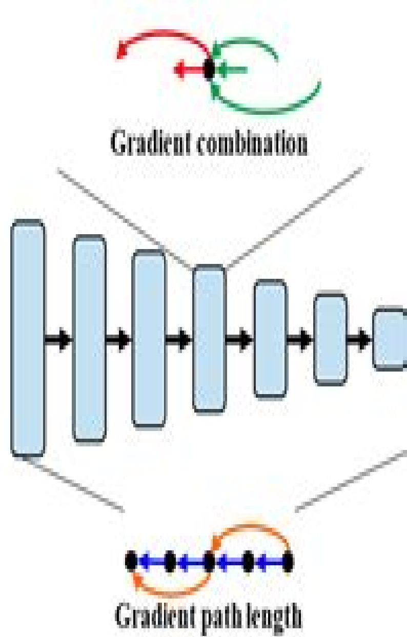
(b) Gradient path design strategies
