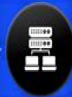
Object-Oriented Database
