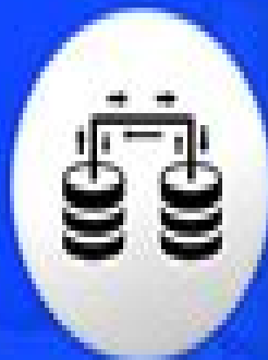
Relational Database
